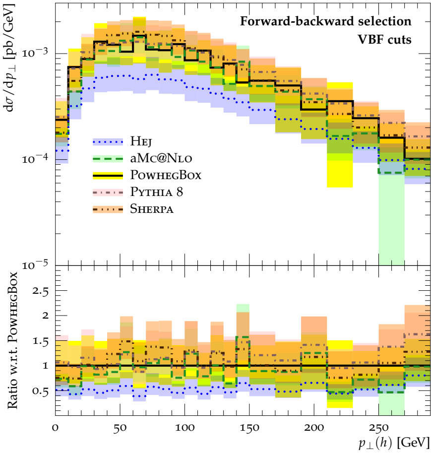
Transverse momentum of the Higgs boson
